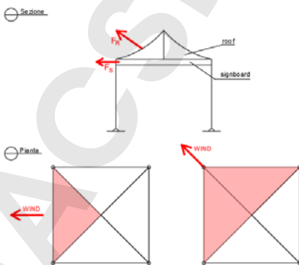
Figure 1 Force application
